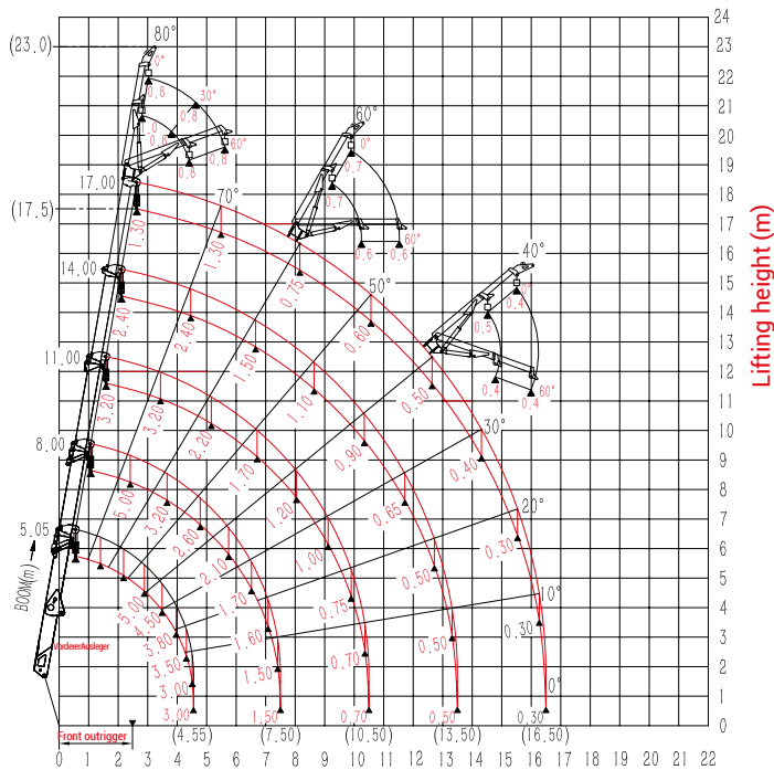
Load diagram (t)
